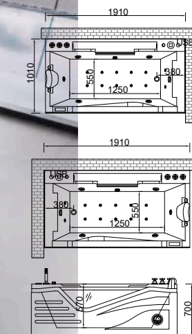
Q325S(L/R) 1910*1010*700mm
