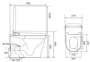
Dimension drawing (size:mm)
