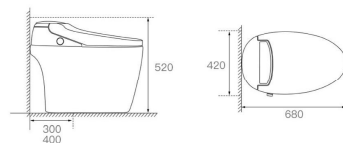
Dimension drawing (size:mm)
