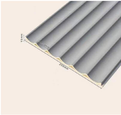
Name: 206 Corrugated board Size: 206x3000x15mm Material: WPC
