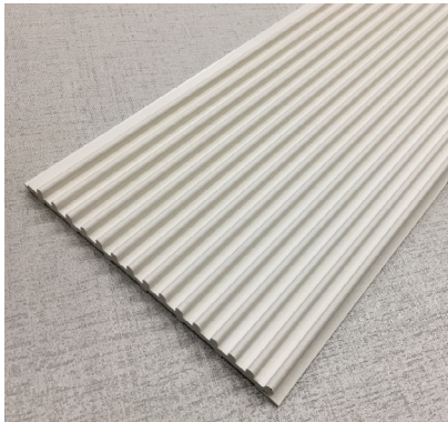
Name: CY#W165 Size: 165x3000x12mm Material: WPC
