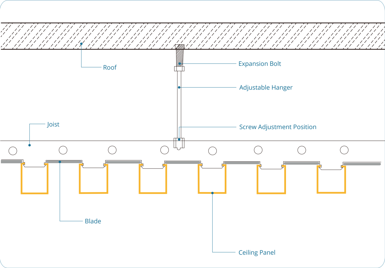
Ceiling Installation Cross-sectional Schematic Diagram
