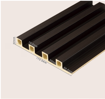
Name: 170 Grille Size: 173.5x3000x22mm Material: WPC
