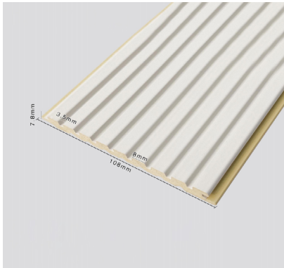
Name: 1039 Premium grille Size: 108x3000x7.8mm Material: WPC
