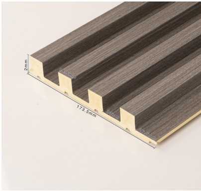
Name: 166 Solid grille Size: 173.5x3000x22mm Material: WPC
