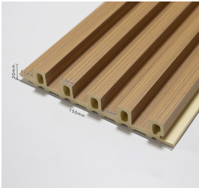
Name: 139 Grille Size: 150x3000x20mm Material: WPC
