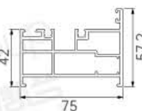
75 大折叠门边框 75 large folding door frame
