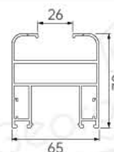
75 大折叠门光企 75 major folding door light enterprises
