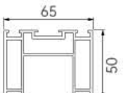
75 大折叠门收口光企 75 fold door closure light enterprise
